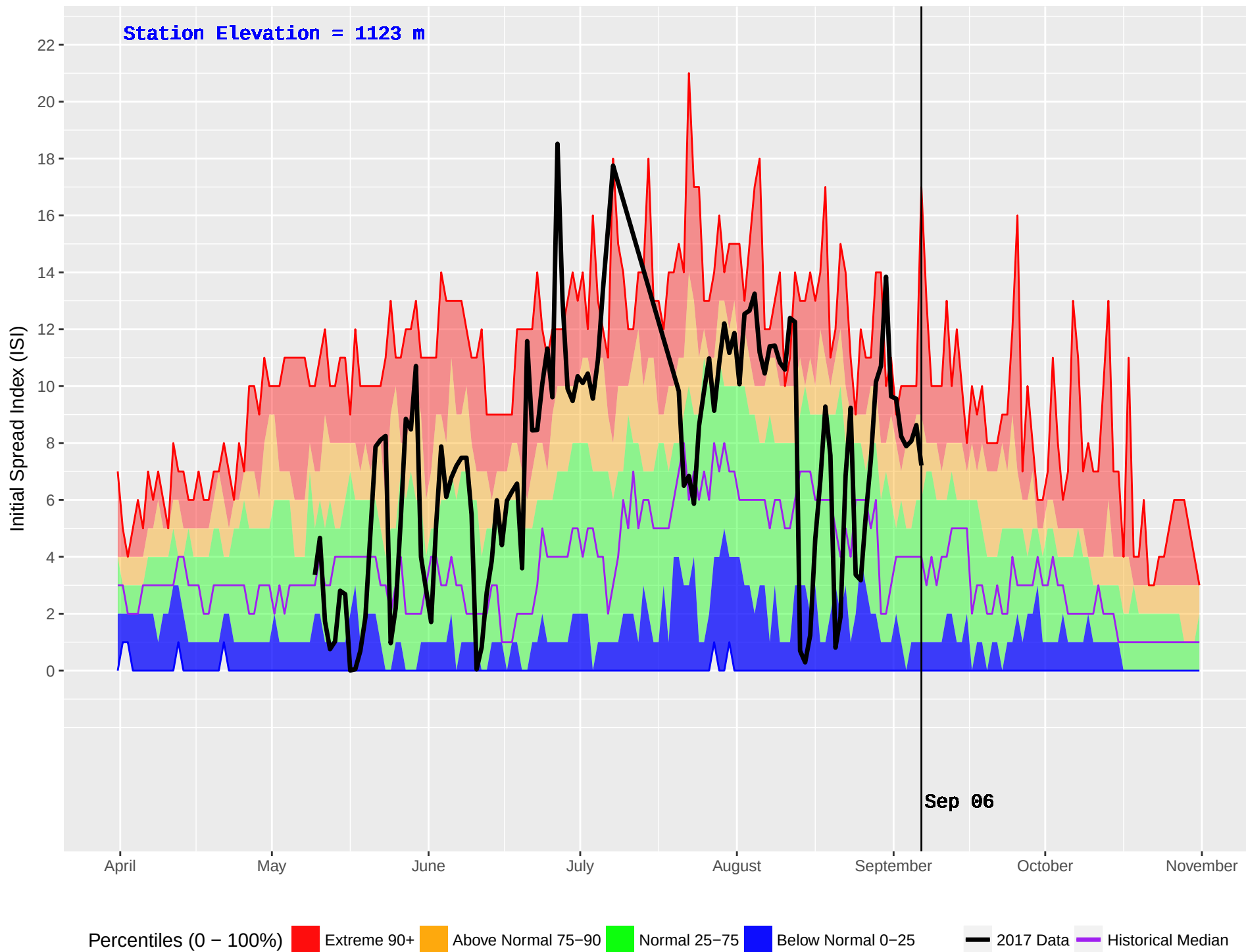
MCLEAN LAKE (311) : Historical (1987–2016) and Current (2017) Noon Initial Spread Index (ISI)
