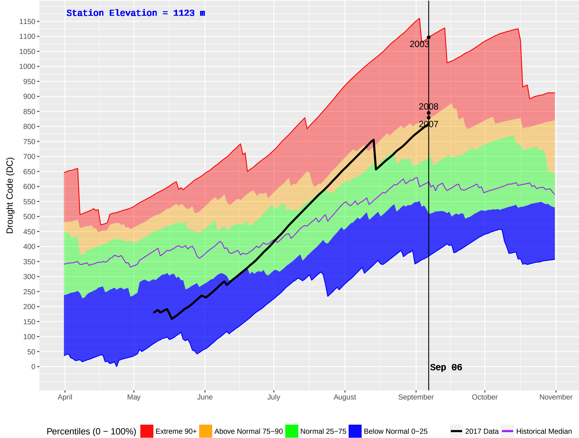
MCLEAN LAKE (311) : Historical (1987–2016) and Current (2017) Noon Drought Code (DC)
