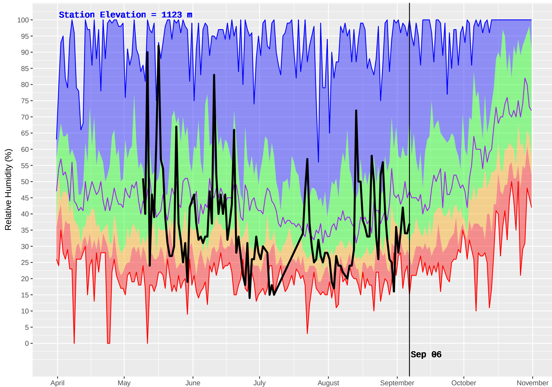
MCLEAN LAKE (311) : Historical (1987–2016) and Current (2017) Noon Relative Humidity
