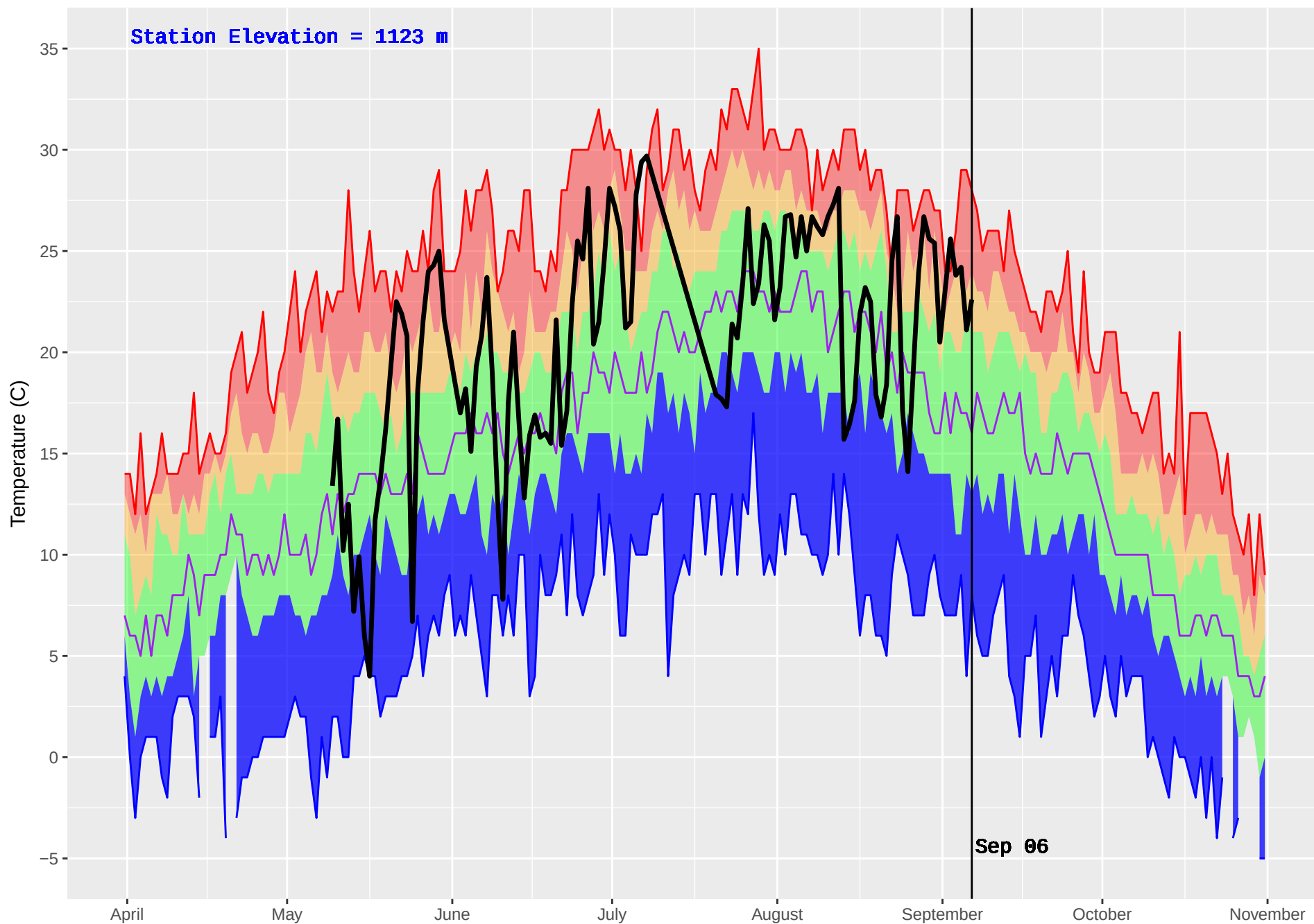
MCLEAN LAKE (311) : Historical (1987–2016) and Current (2017) Noon Temperature
