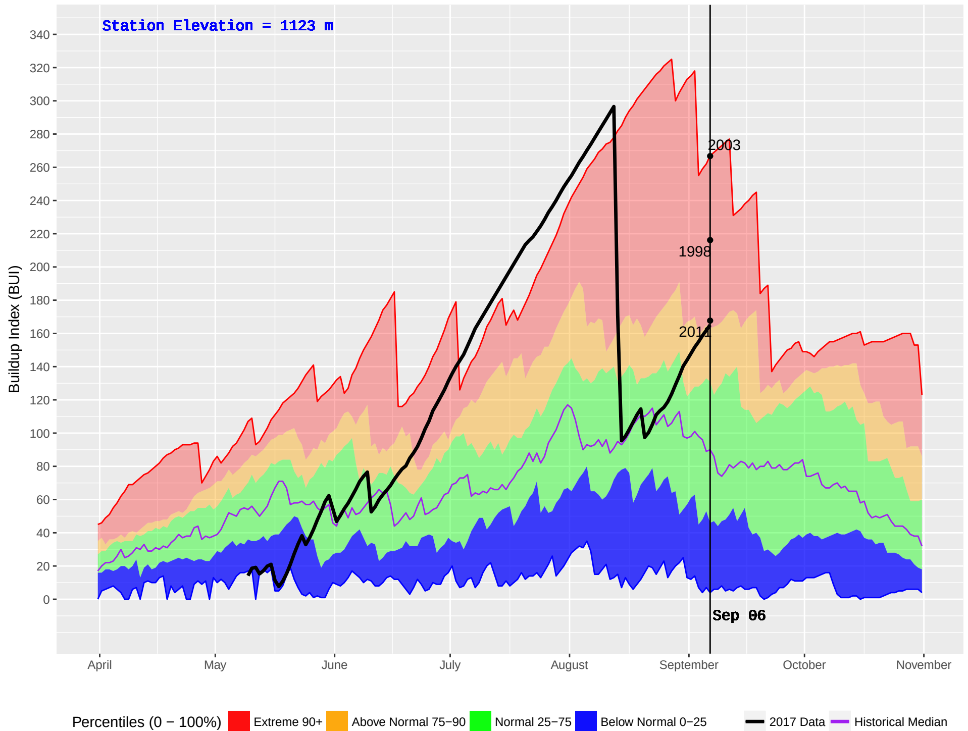
MCLEAN LAKE (311) : Historical (1987–2016) and Current (2017) Noon Buildup Index (BUI)
