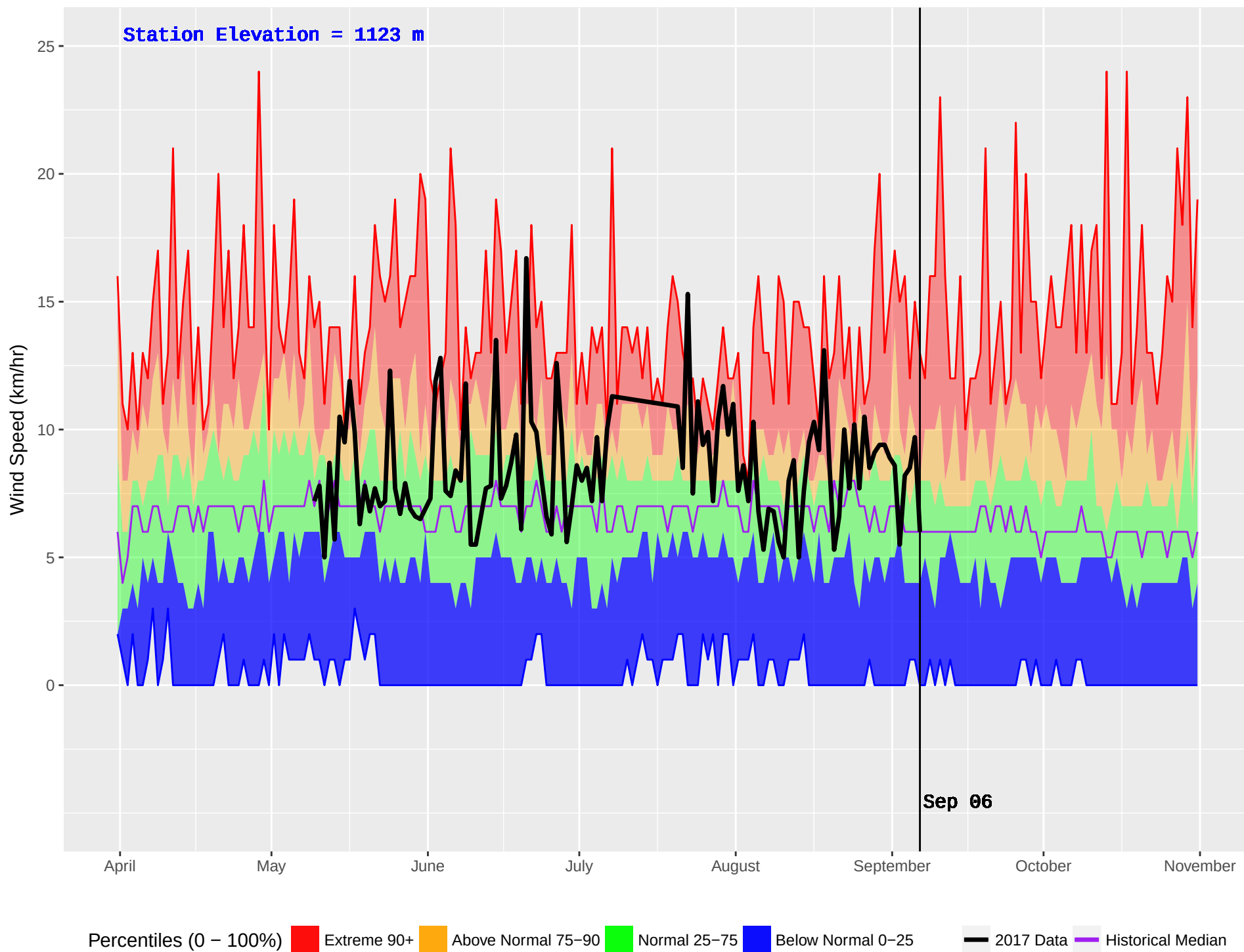
MCLEAN LAKE (311) : Historical (1987–2016) and Current (2017) Noon Wind Speed
